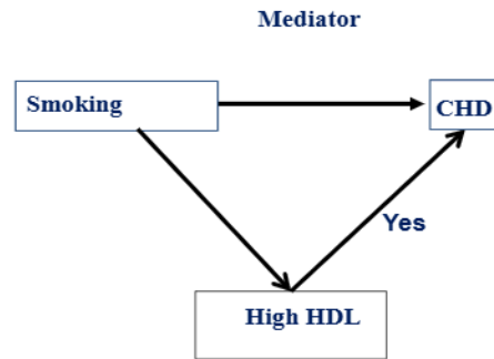
Fig. 2: Mediator
