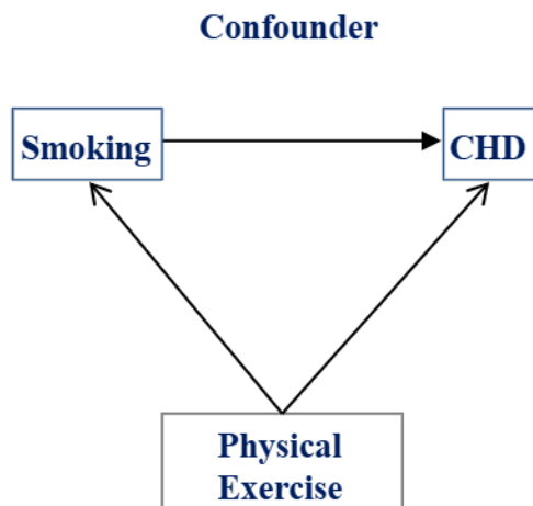
Fig. 1: Confounder
