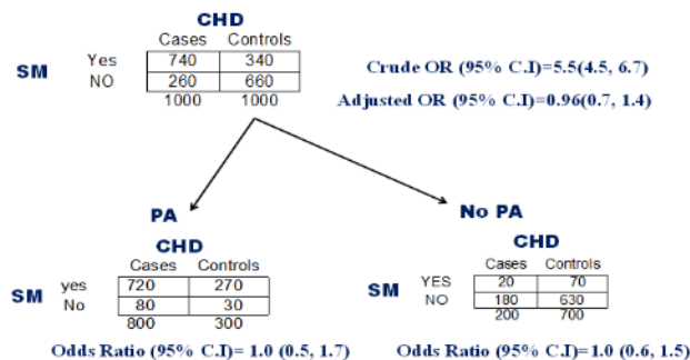
Fig. 6: Only confounder
